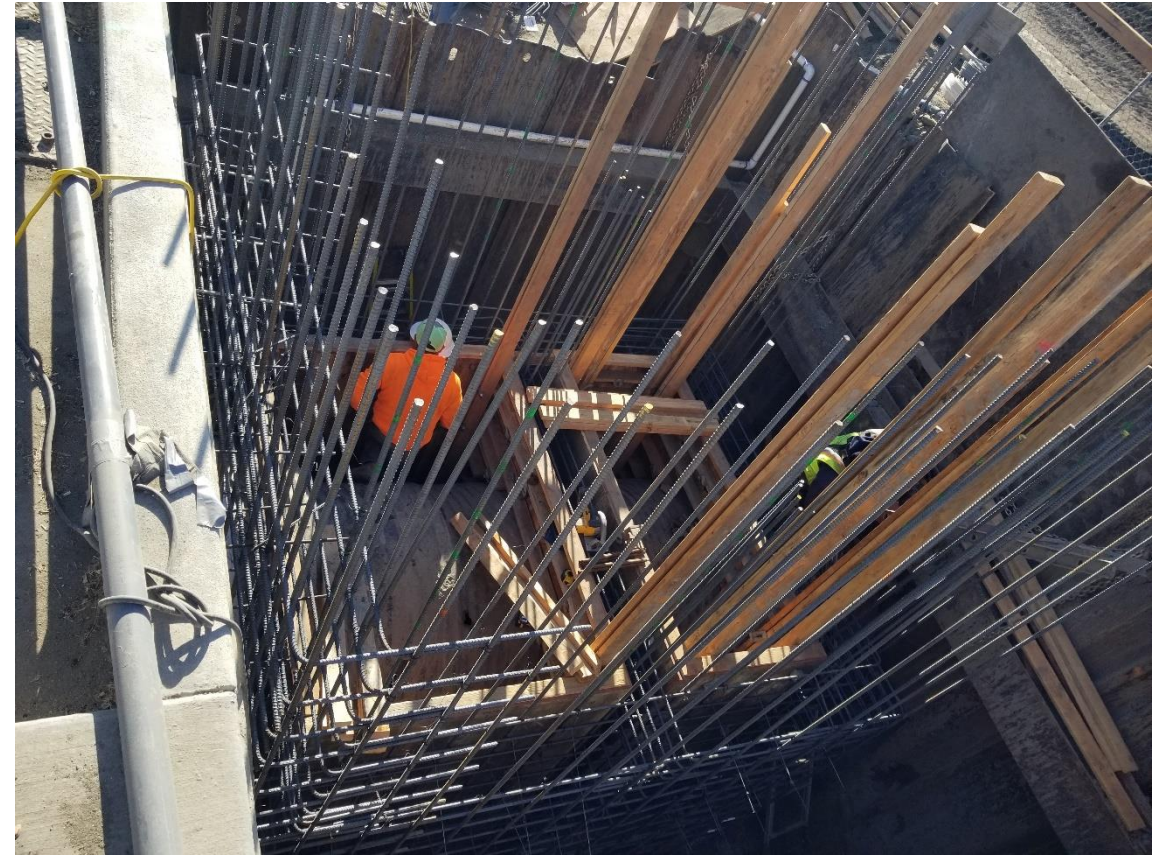
INSTALLING REBAR & FORMS IN SW DIVERSION VAULT
