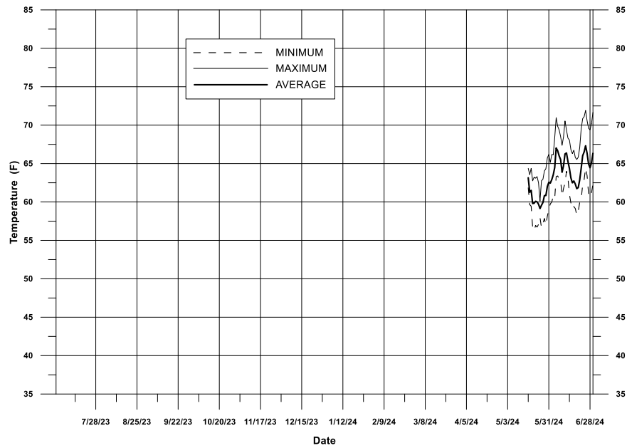
Figure III-2 Daily temperatures recorded from a continuous temperature data logger at the Sleepy Hollow Weir (SHW) station during RY 2024
