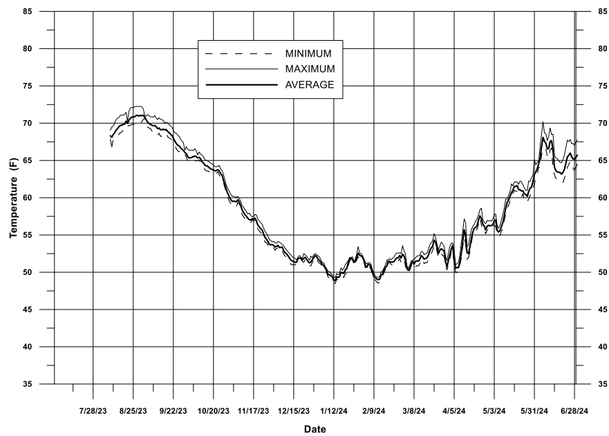
Figure III-3 Daily temperatures recorded from a continuous temperature data logger at the Below Los Padres (BLP) station during RY 2024
