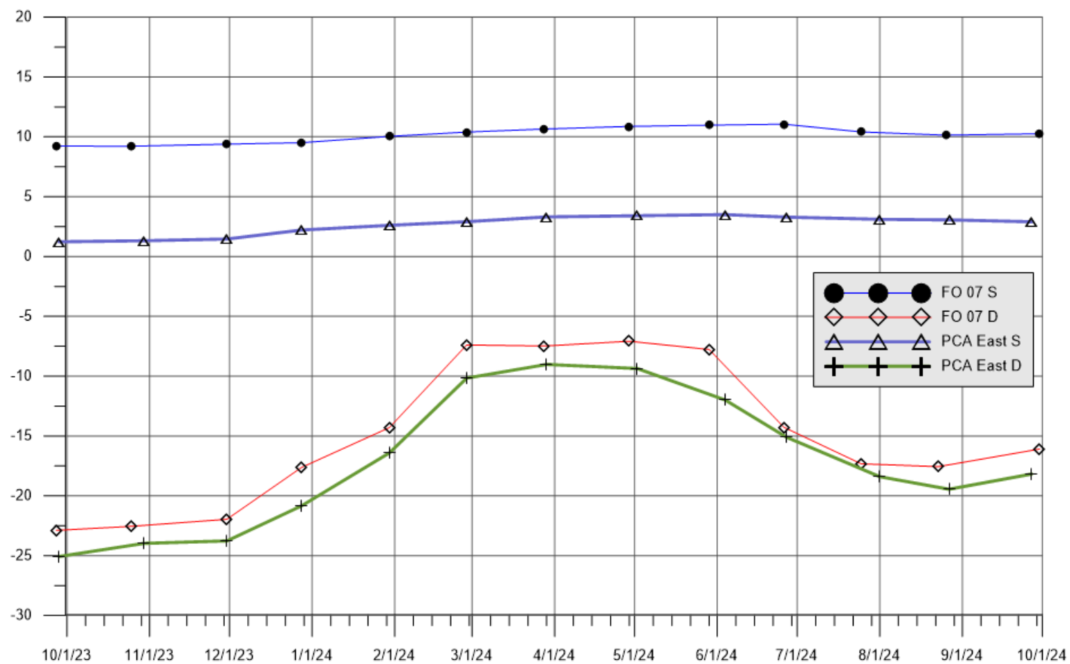
Figure IV-2 Hydrographs of PCA East and FO 07
