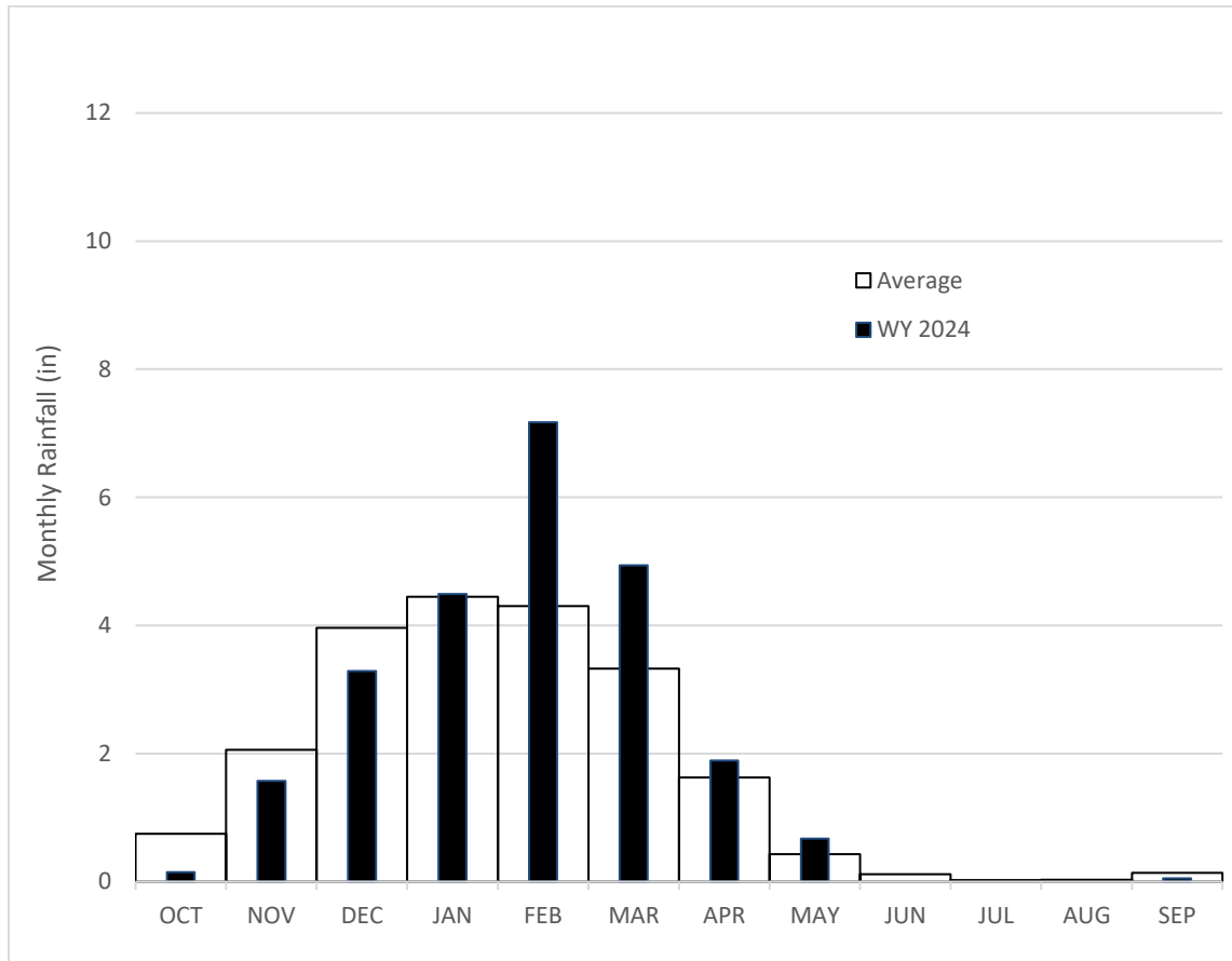
Figure II-2 Monthly Distribution of Rainfall at San Clemente Reservoir Site Water Year 2024 Compared to 1922-2024 Long-Term Average
