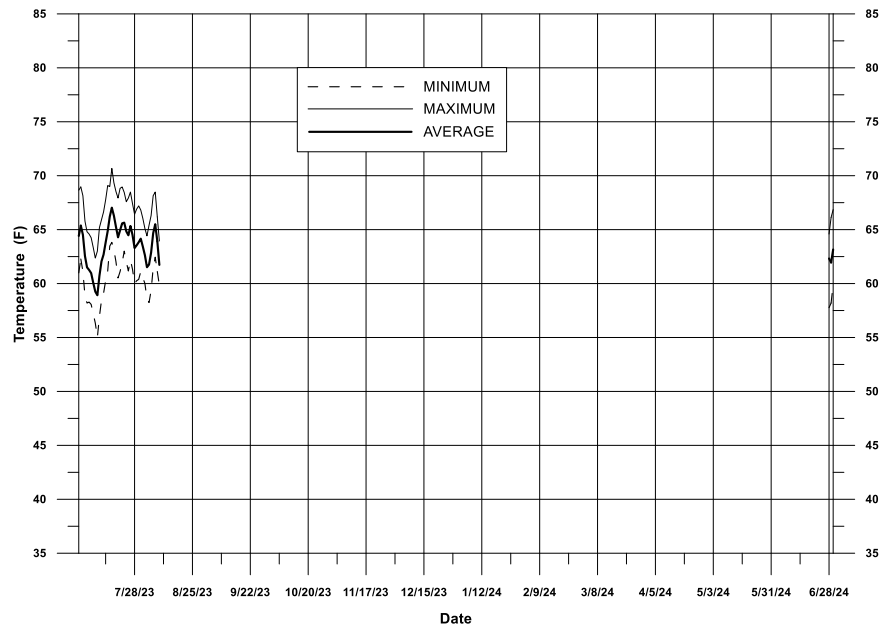
Figure III-4 Daily temperatures recorded from a continuous temperature data logger at the Above Los Padres (ALP) station during RY 2024
