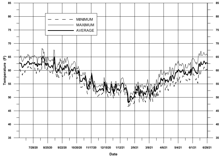
Figure III-2 Daily temperatures recorded from a continuous temperature data logger at the Garland Park (GAR) station during RY 2021
