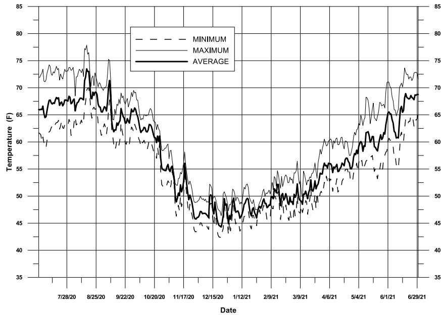
Figure III-3 Daily temperatures recorded from a continuous temperature data logger at the Sleepy Hollow Weir (SHW) station during RY 2021
