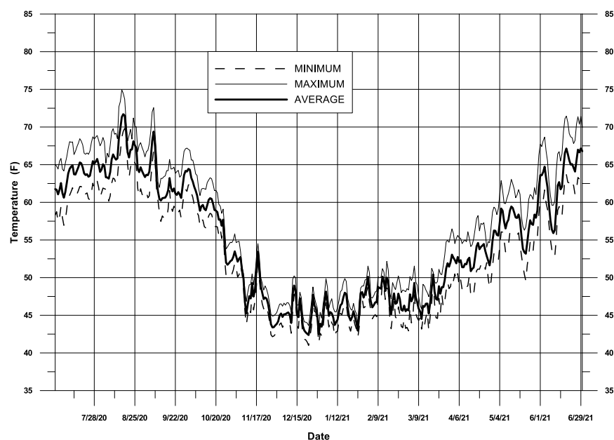
Figure III-6 Daily temperatures recorded from a continuous temperature data logger at the Above Los Padres (ALP) station during RY 2021
