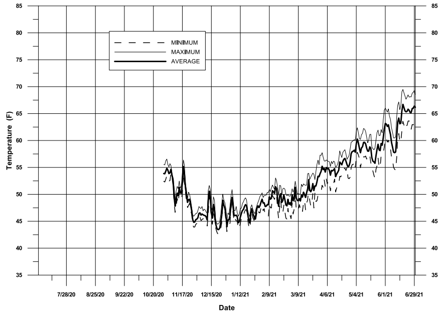
Figure III-5 Daily temperatures recorded from a continuous temperature data logger at the Below Los Padres (BLP) station during RY 2021
