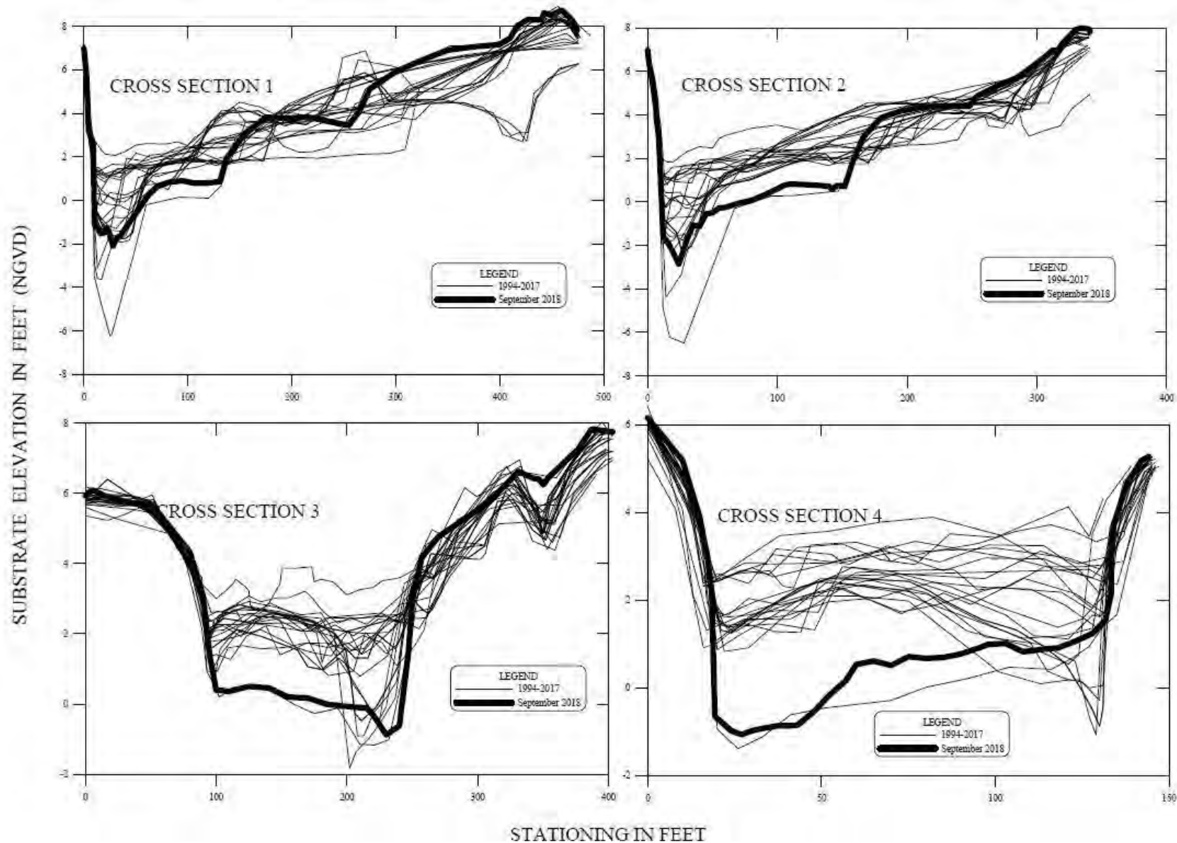
Figure XVIII-2 Carmel River Lagoon Cross Sections 1 through 4, based on Annual Surveys 1994-2018
