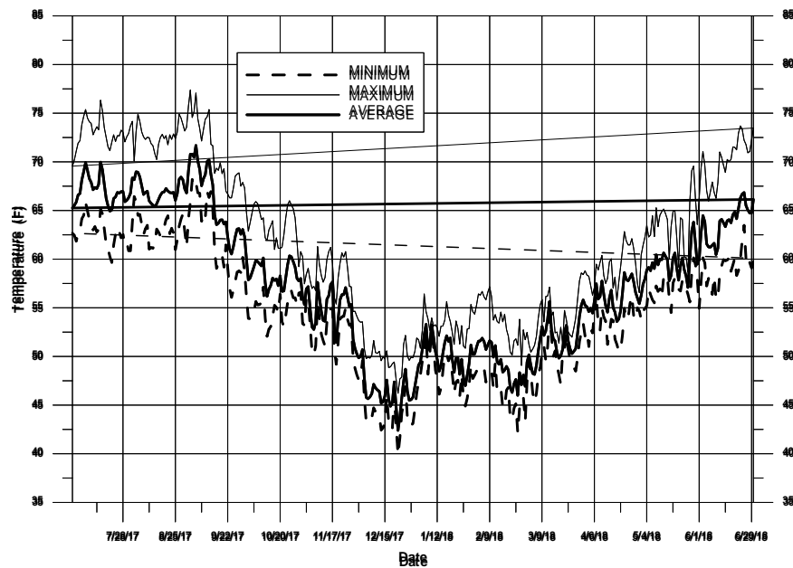
Figure III-3 Daily temperatures recorded from a continuous temperature data logger at the Sleepy Hollow Weir (SHW) station during RY 2018
