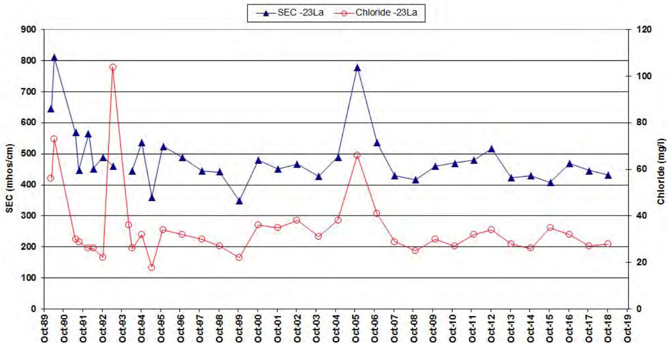
Figure IV-6 WATER-QUALITY RESULTS Reimers #1 - 16S/1E-23La River Mile 6.72
