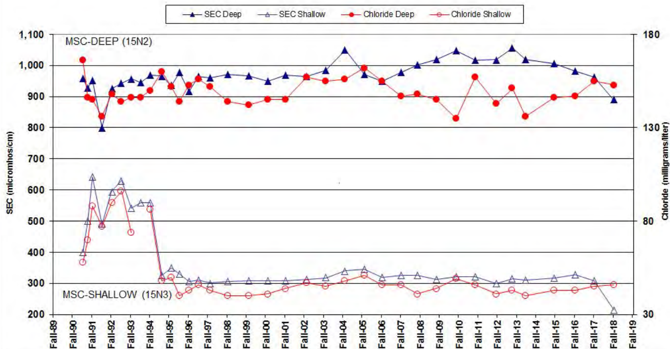
Figure IV - 8 WATER-QUALITY RESULTS MSC (Monterey Sand Company) 15S/1E-15N2 (deep) and 15S/1E-15N3 (shallow)
