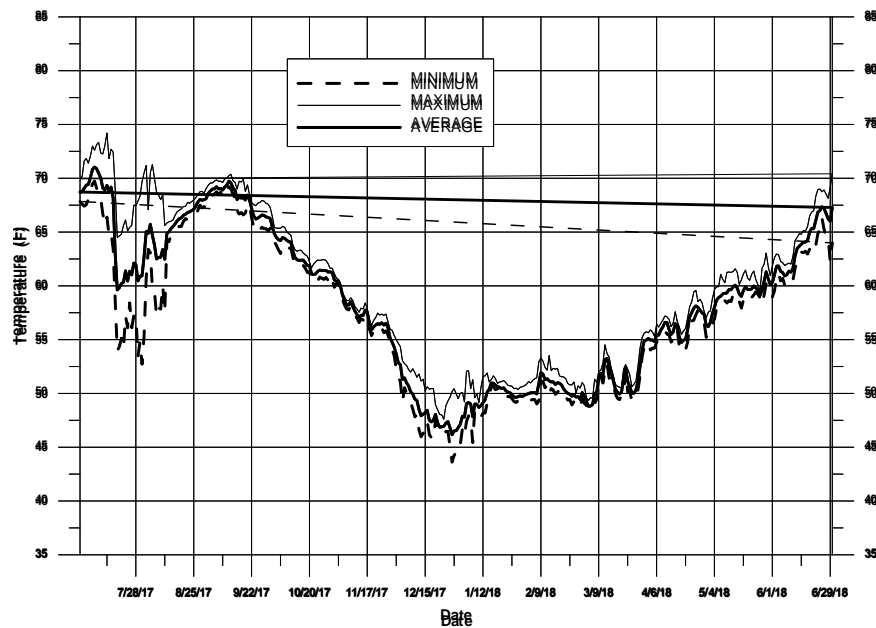
Figure III-5 Daily temperatures recorded from a continuous temperature data logger at the Below Los Padres (BLP) station during RY 2018
