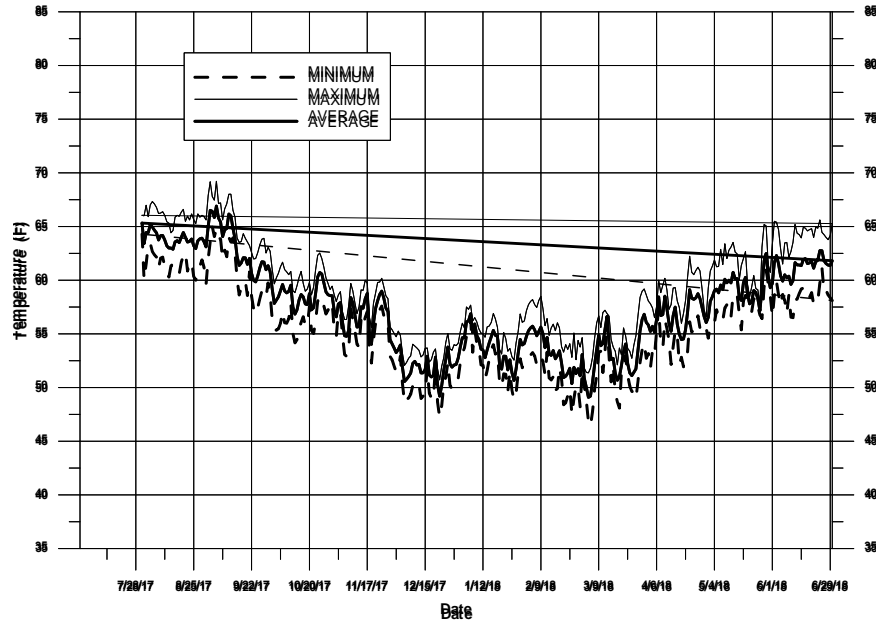
Figure III-2 Daily temperatures recorded from a continuous temperature data logger at the Garland Park (GAR) station during RY 2018
