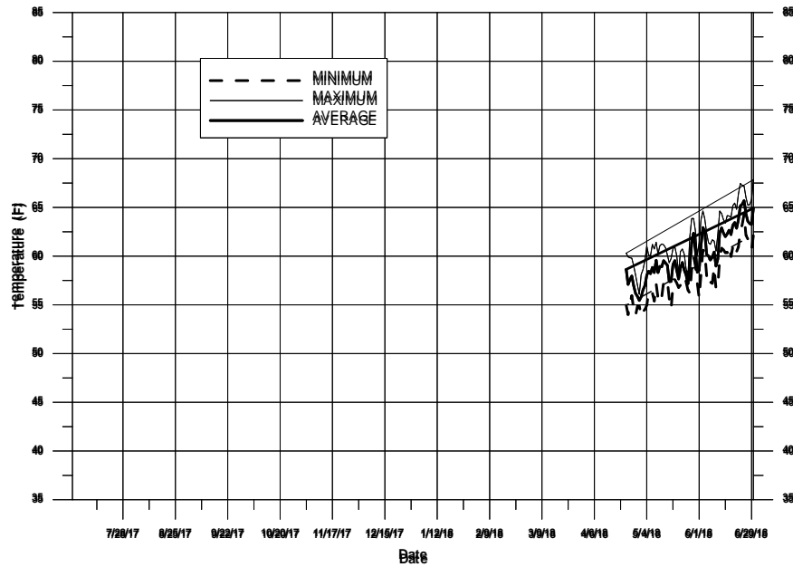
Figure III-4 Daily temperatures recorded from a continuous temperature data logger at the above San Clemente (ASC) station during RY 2018
