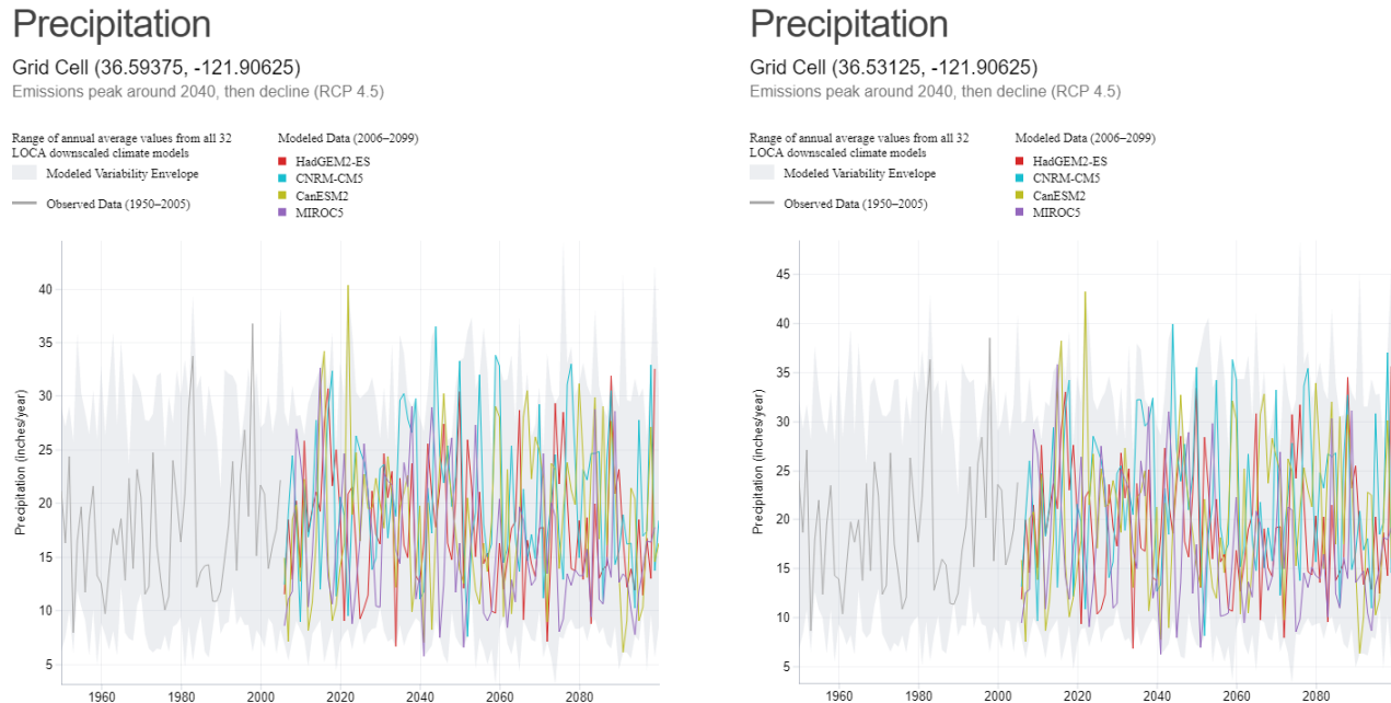
Figure 15-3: Projected Average Rainfall in Monterey (Left) and Carmel Area (Right)
