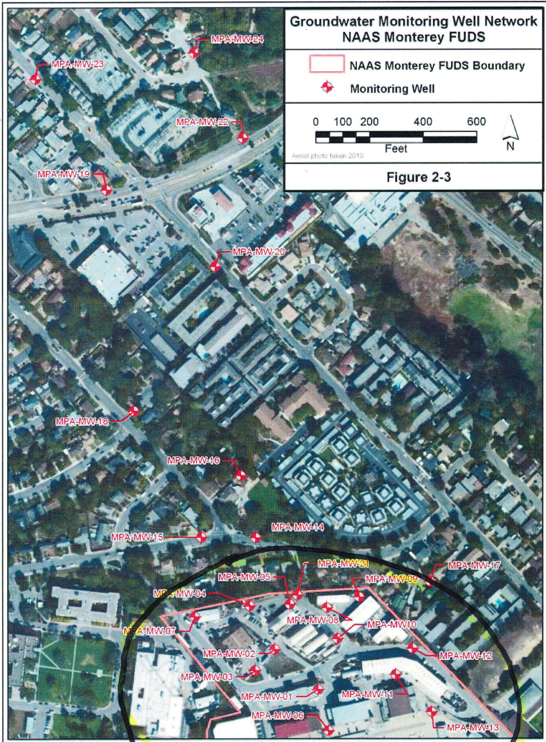
Figure 2-3. Groundwater Monitoring Well Network, NAAS Monterey FUDS
