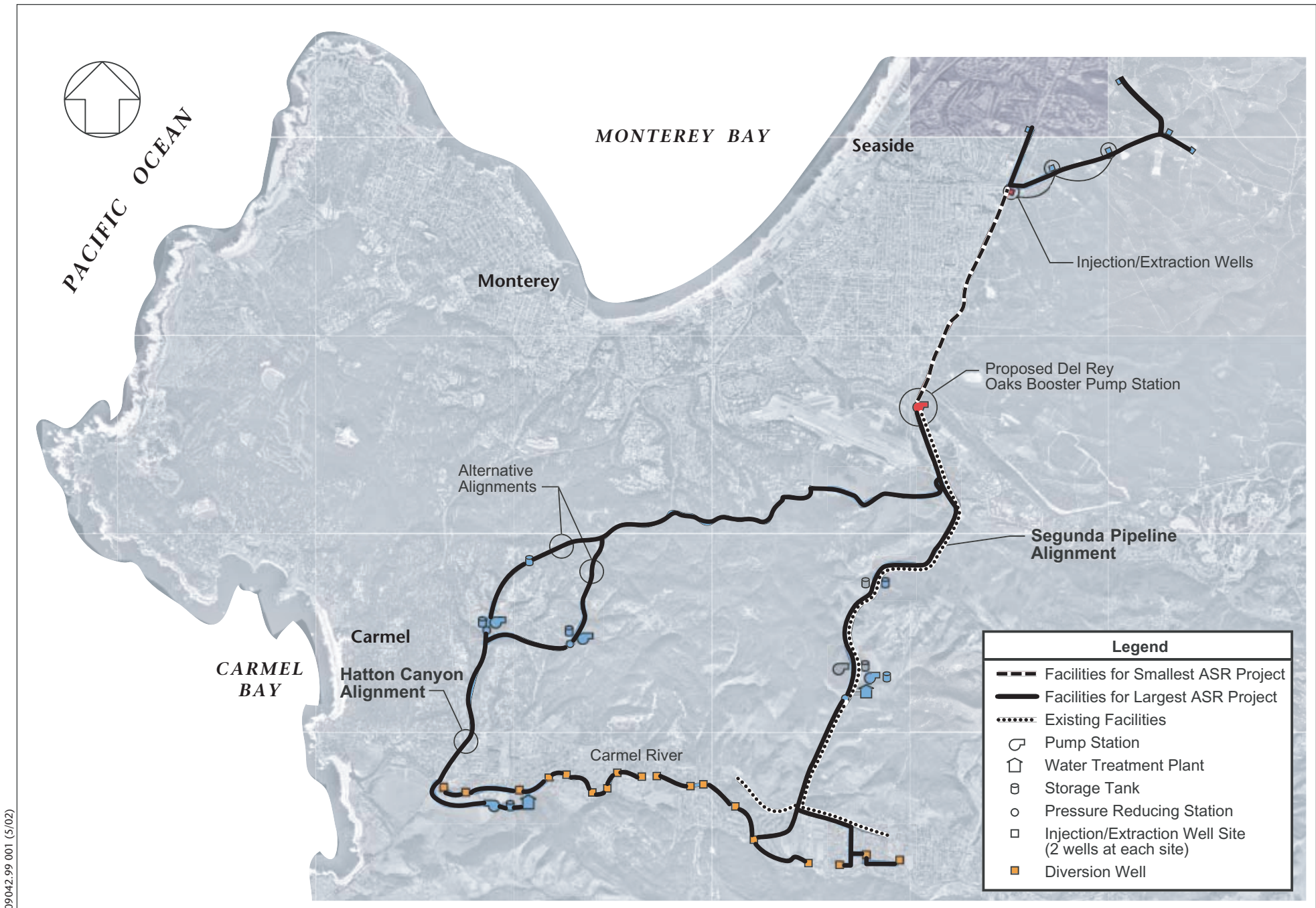
Figure 2 Aquifer Storage and Recovery Project Facilities
