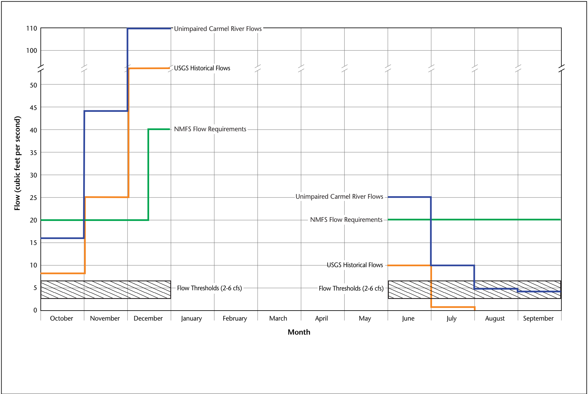
Figure C-2 Summary Comparison of Flow Criteria for Carmel River Steelhead Rearing Capacity in Normal Years (June – December)
