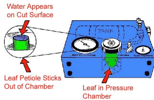
Figure 3. Pressure Bomb Instrument Illustration Courtesy of PMS Instrument Co.
