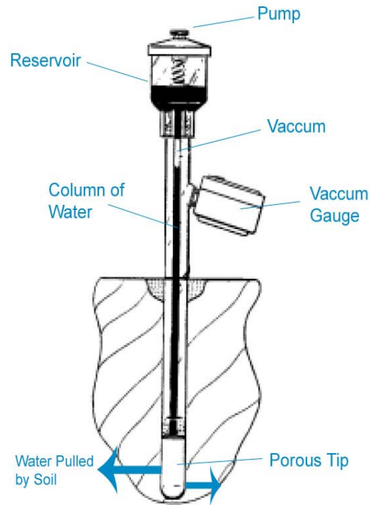
Figure 2. Tensiometer
