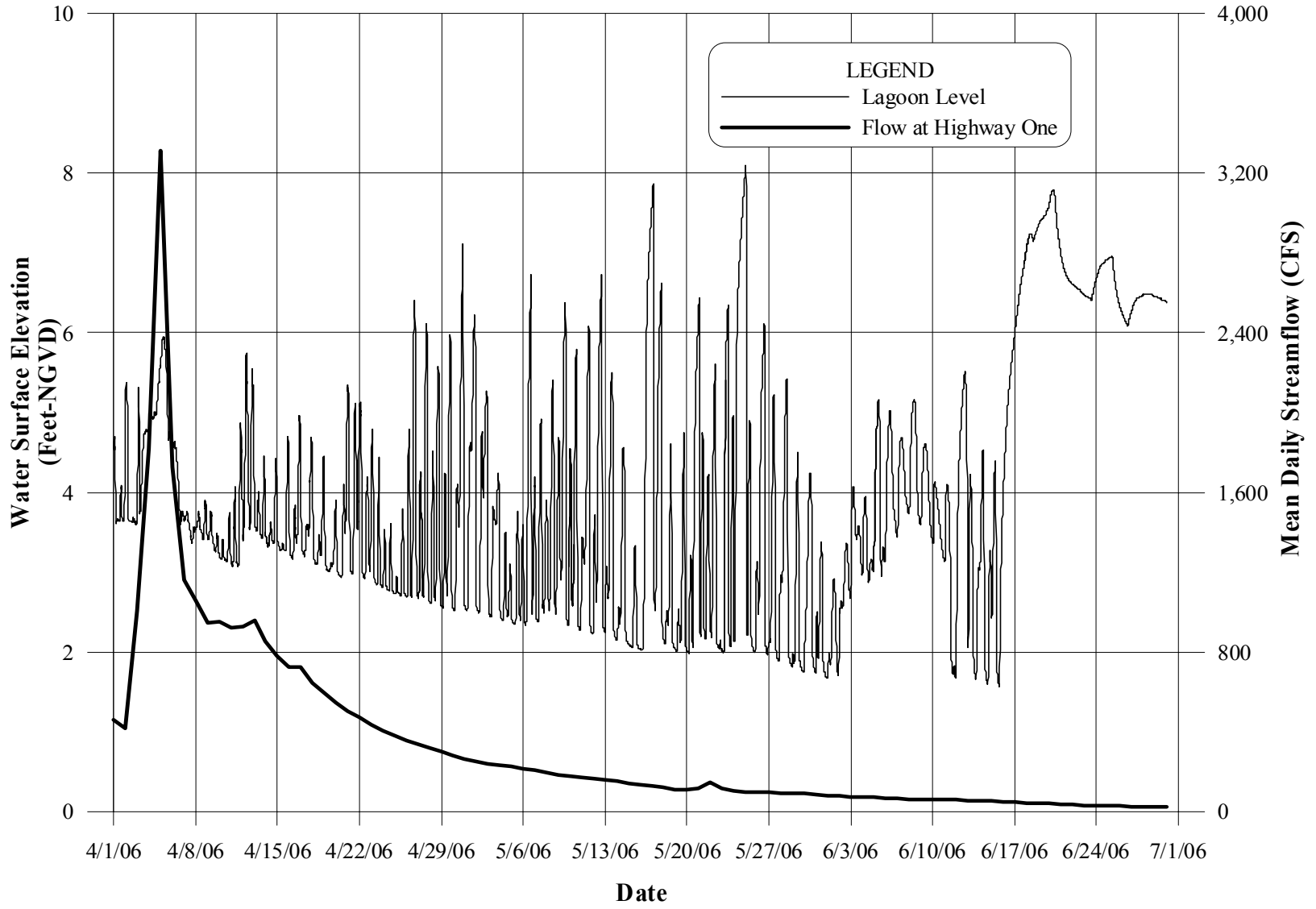
Figure IX-1 Water Surface Elevation in the Carmel River Lagoon and Streamflow at the Highway One Bridge: April through June 2006
