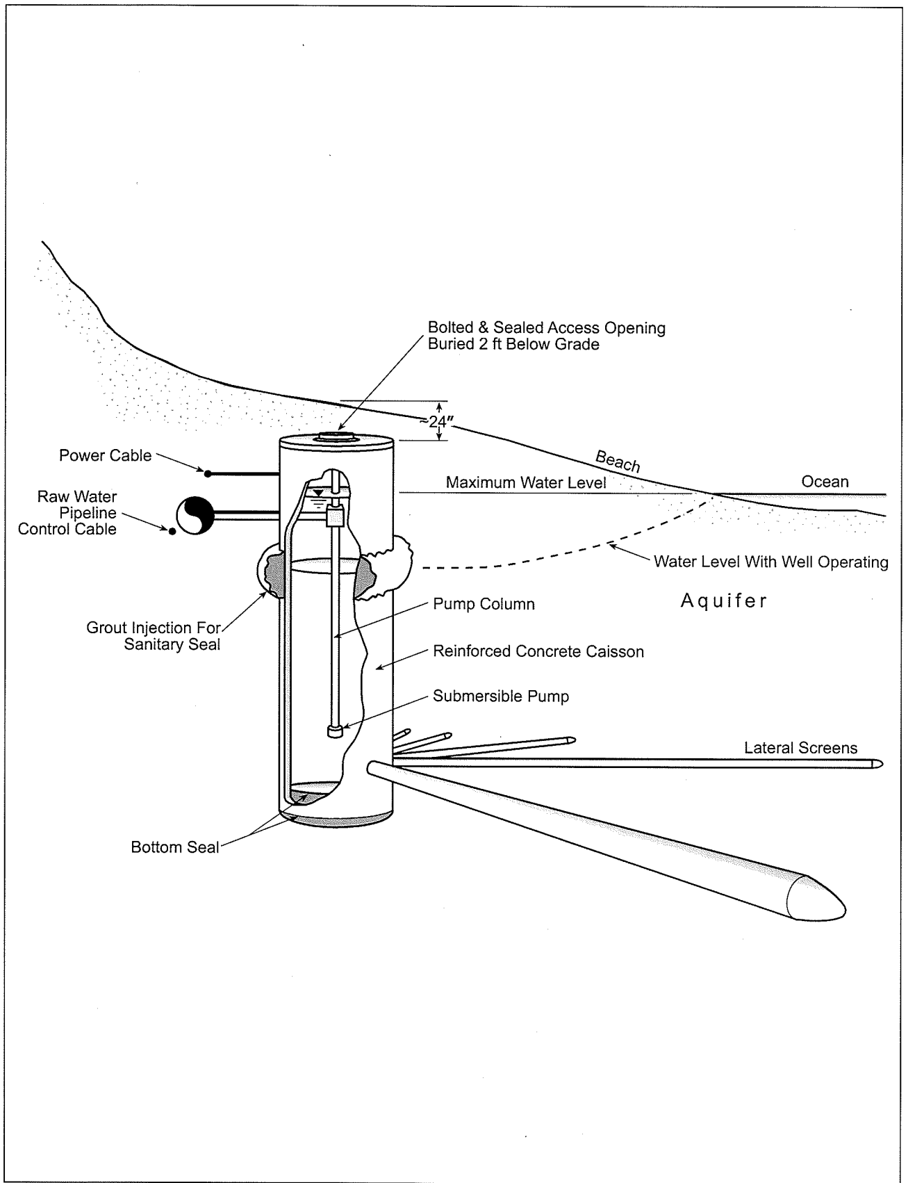
Figure 6 Radial Collector Well Conceptual Layout Sand City Desalination Project
