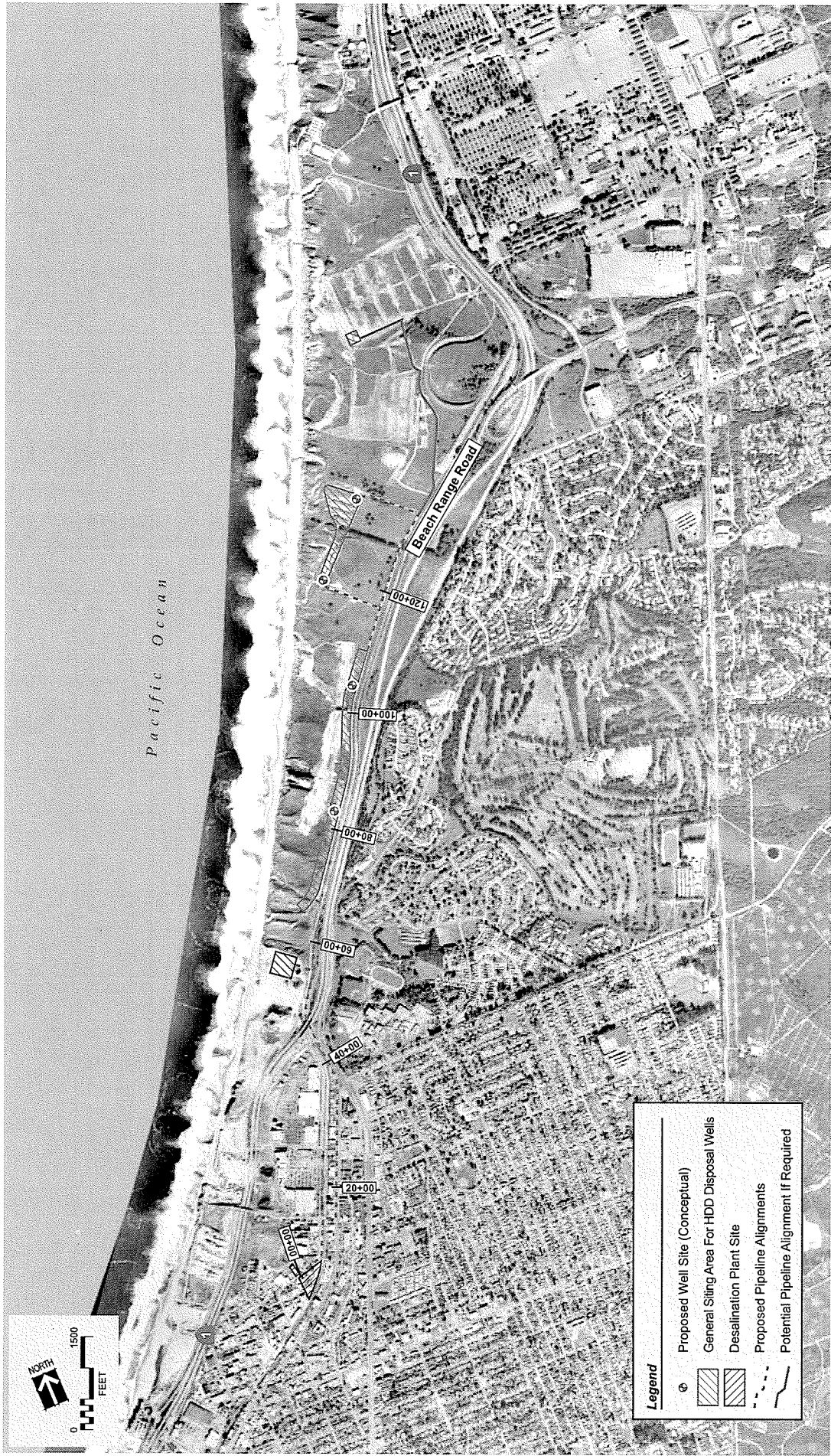
Figure 7 HDD Well Brine Disposal System Siting Areas & Pipeline Alignments Sand City Desalination Project
