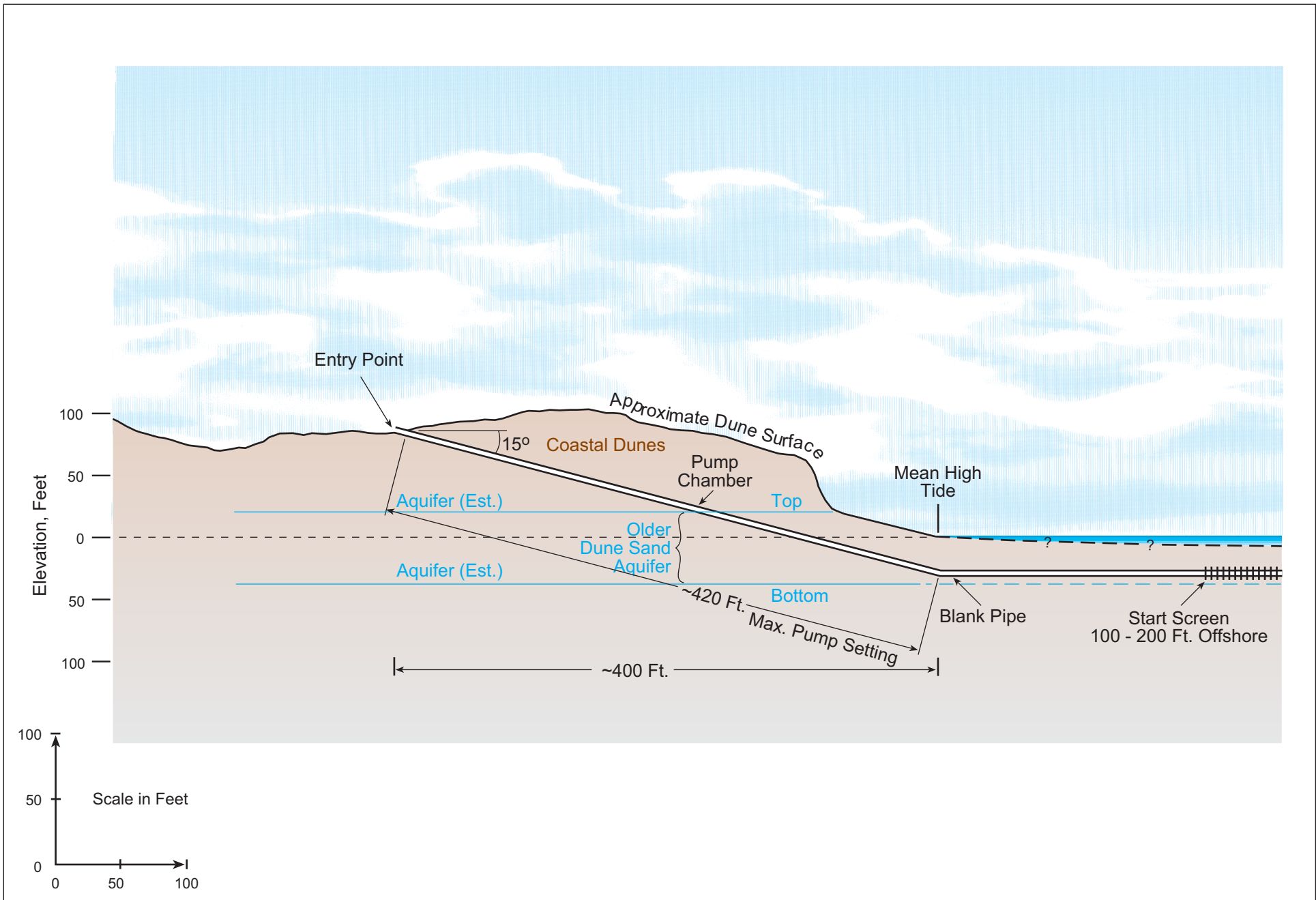
Figure 4 Conceptual Cross-Section For An HDD Well Sand City Desalination Project
